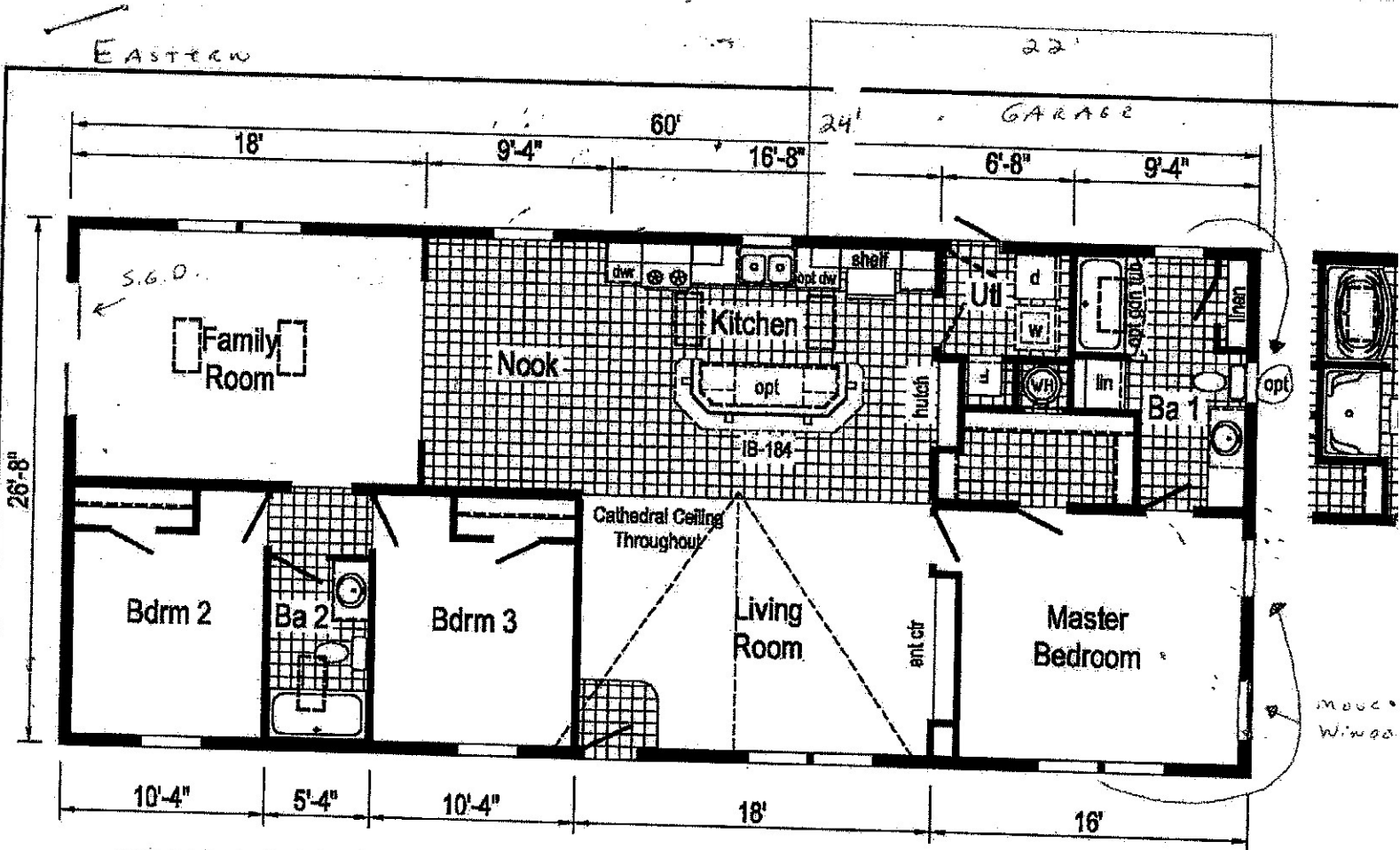
TD118-A 2860 Approx. 1600 Sq. Ft.
